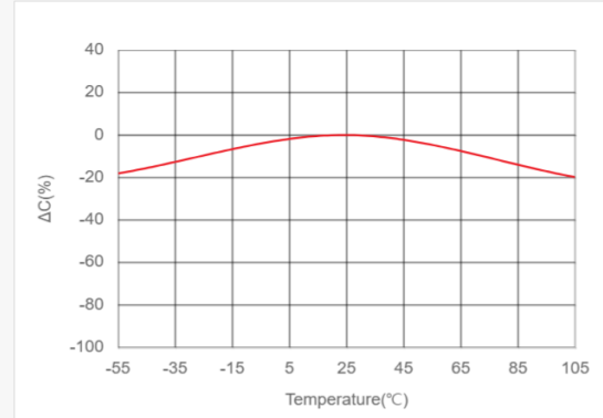
Temperature Characteristics of Capacitance(TCC) LCR meter, 0.12kHz, 0.12Vrms
